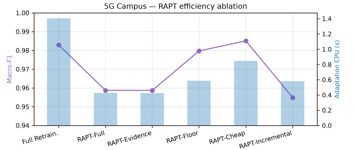
Fig. 5. Ablation ladder comparing the different configurations of RAPT, evaluated on the 5G Campus stream. As shown, RAPT-Cheap matches the full retrainer in terms of macro-F1 at around 40% less adaptation CPU, whereas RAPT-Incremental performs worse on both accuracy and cost.
